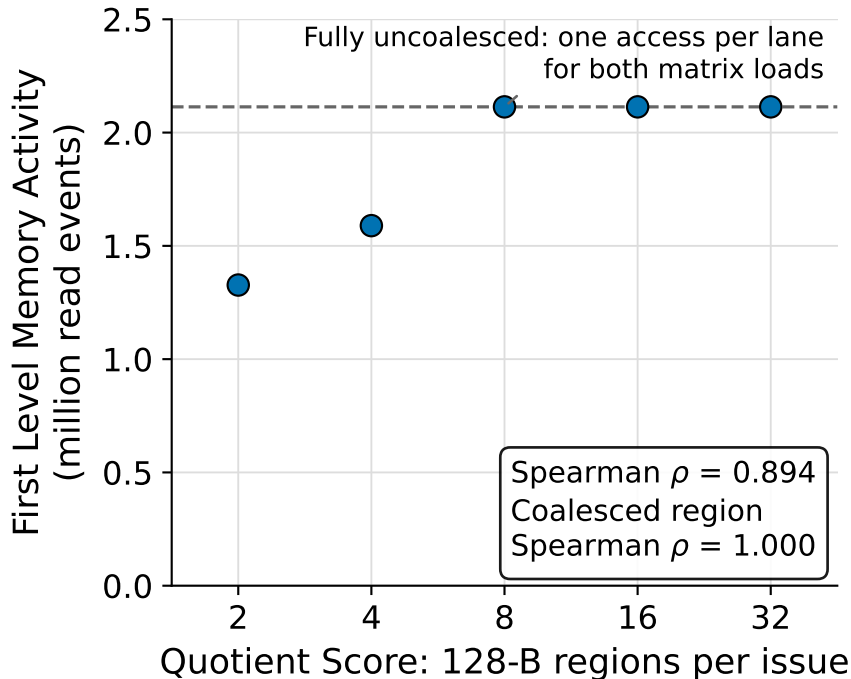
Quotient Score versus First Level Memory Activity (read events) for GESUMMV Kernel on NVIDIA H100
