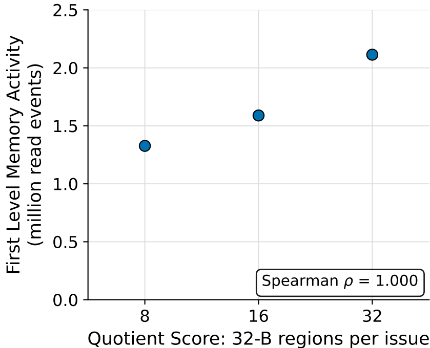
Quotient Score versus First Level Memory Activity (read events) for GESUMMV Kernel on NVIDIA H100
