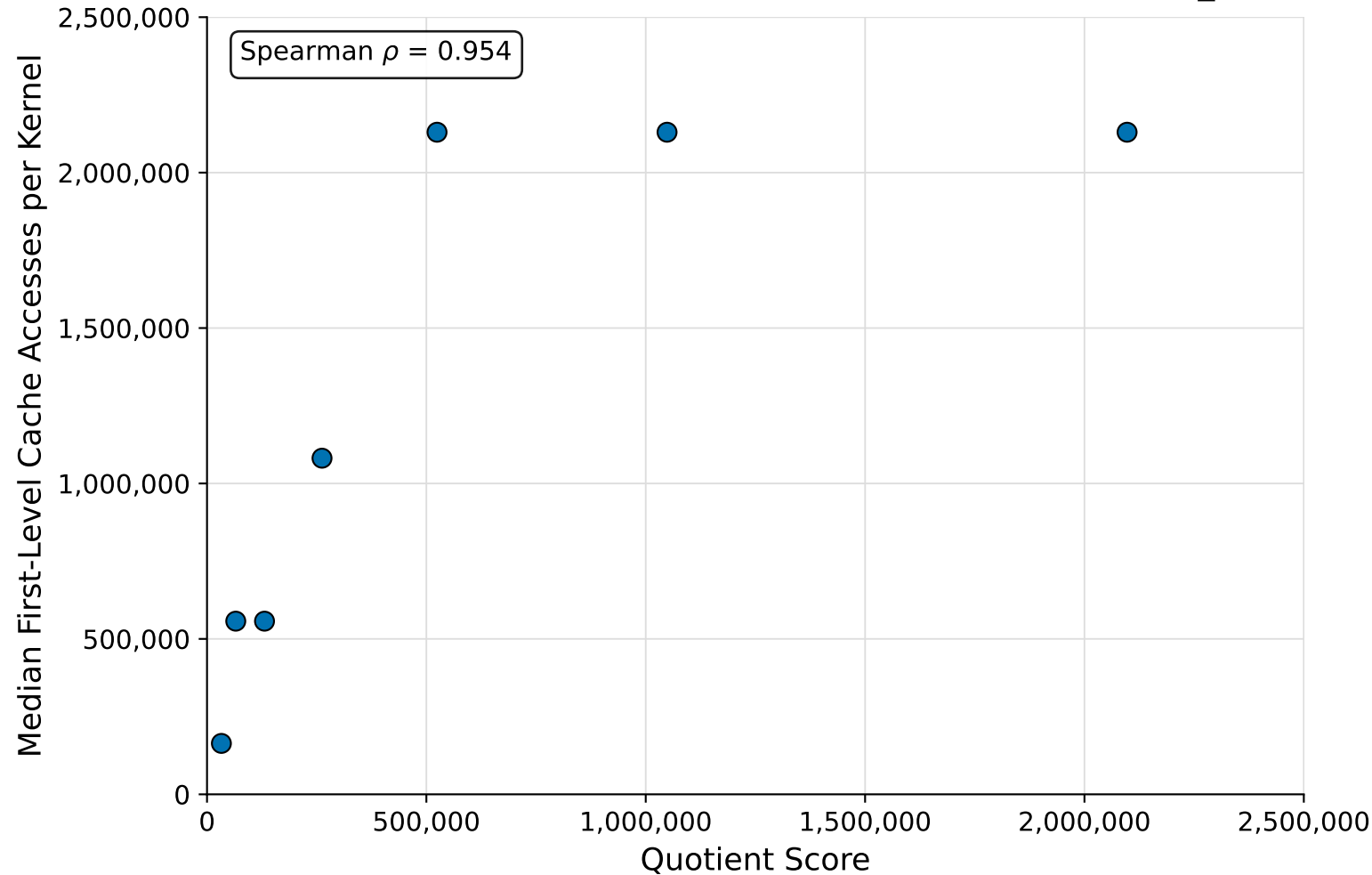
Quotient Score versus First-level Cache Accesses for EMBEDDING_BAG Kernel
