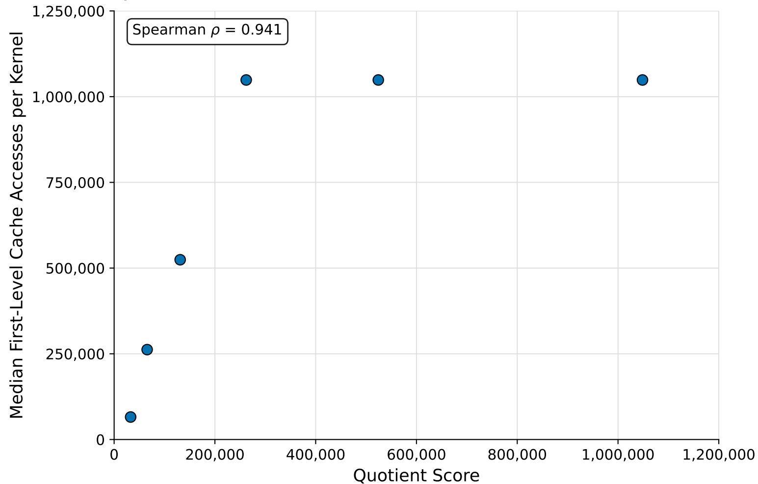
Quotient Score versus First-level Cache Accesses for GEMV Kernel
