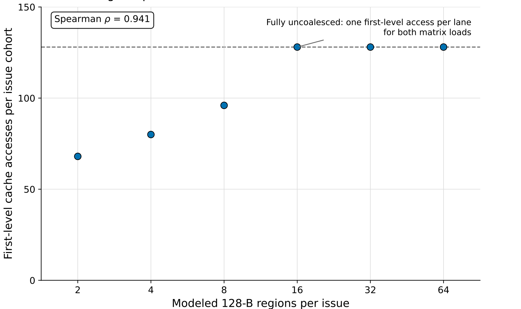
Modeled 128-B Regions per Issue versus First-level Cache Accesses for GESUMMV Kernel
