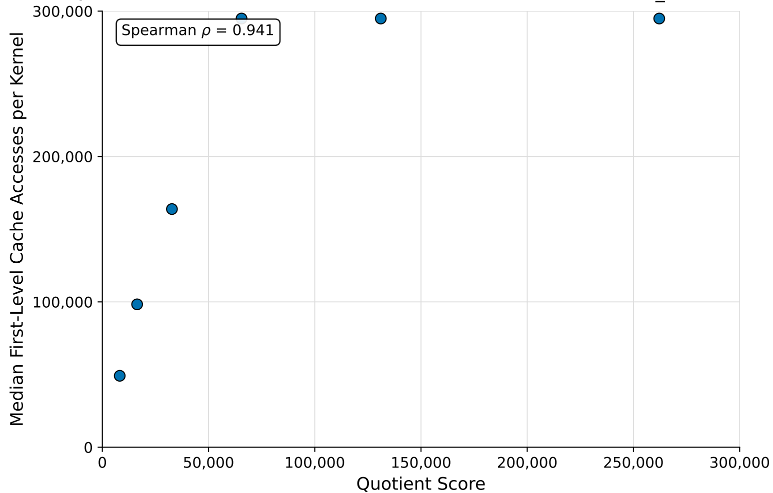
Quotient Score versus First-level Cache Accesses for SOFTMAX_BIAS Kernel
