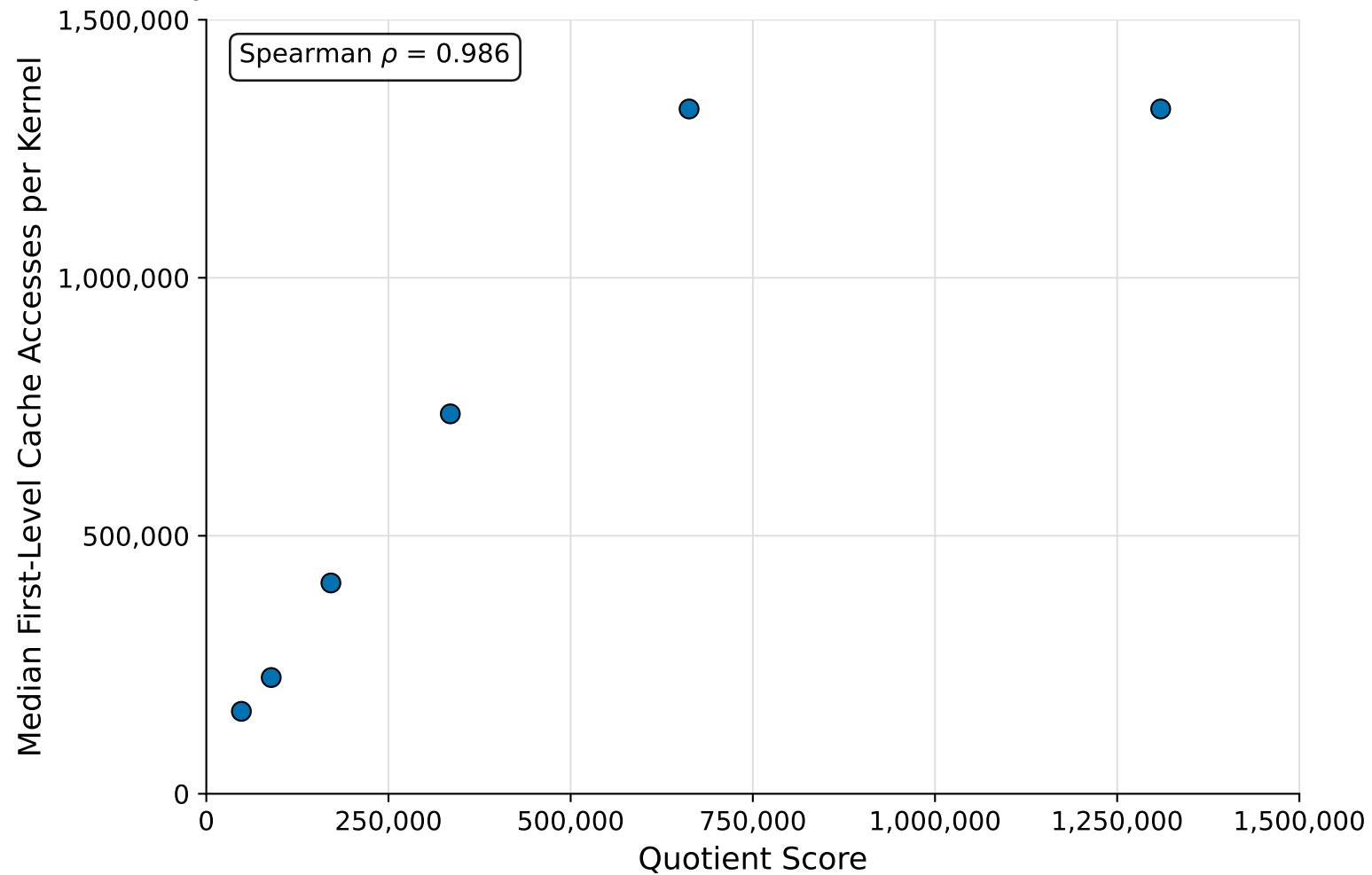
Quotient Score versus First-level Cache Accesses for STENCIL5 Kernel
