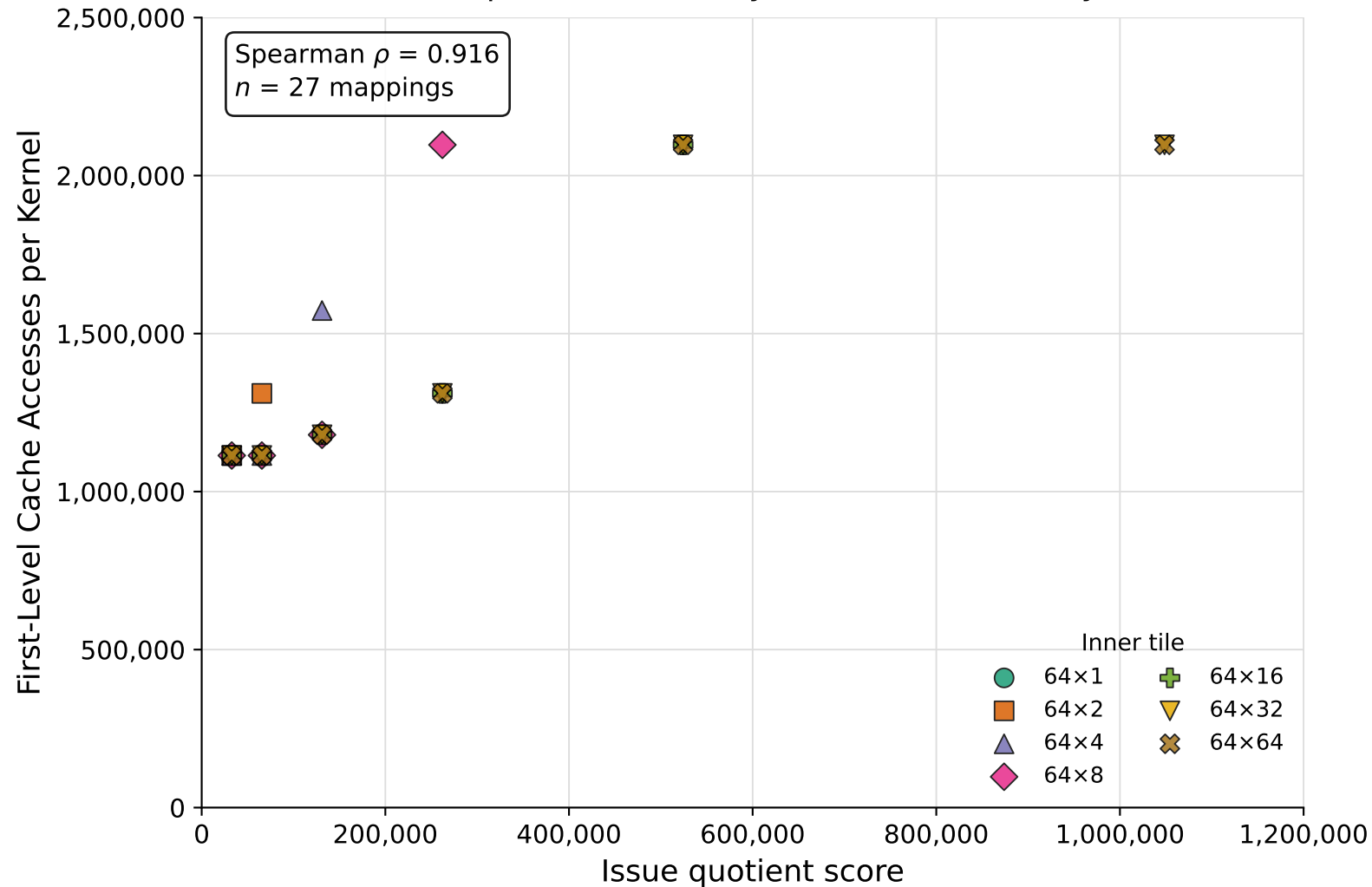
GESUMMV: persistent tile layouts versus memory traffic
