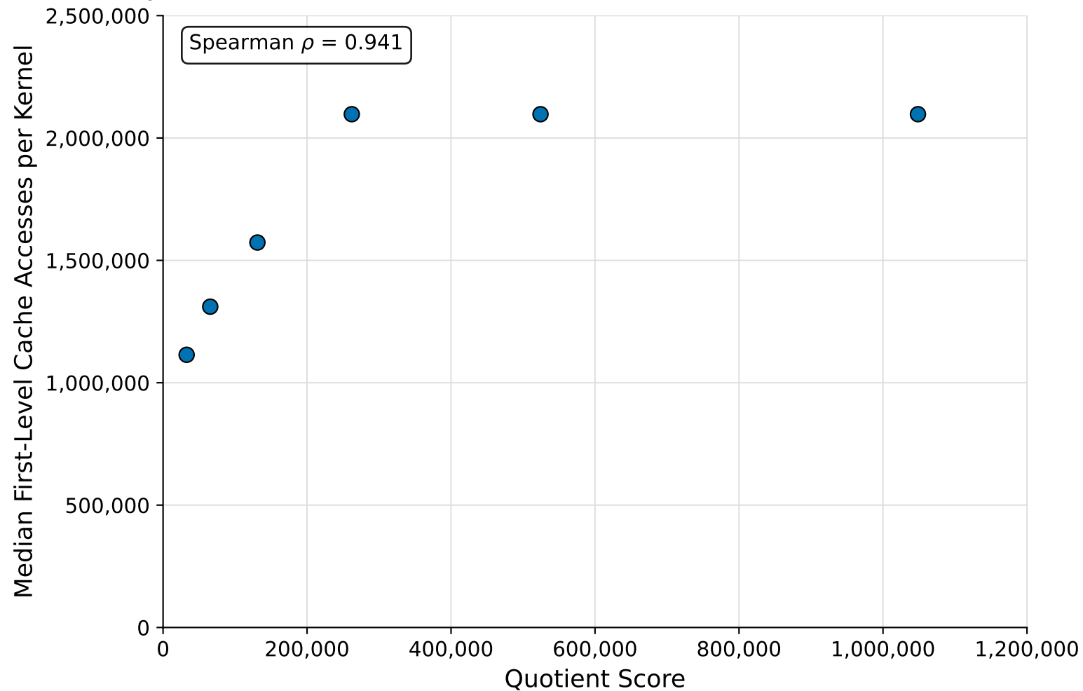
Quotient Score versus First-level Cache Accesses for GESUMMV Kernel
