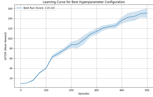
(b) Off-Policy Learning Curve
