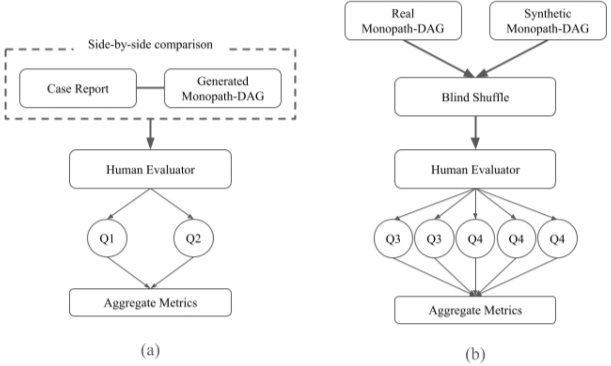
Fig. A1: Human evaluation schematics for (a) fidelity and (b) synthetic graph assessments.
