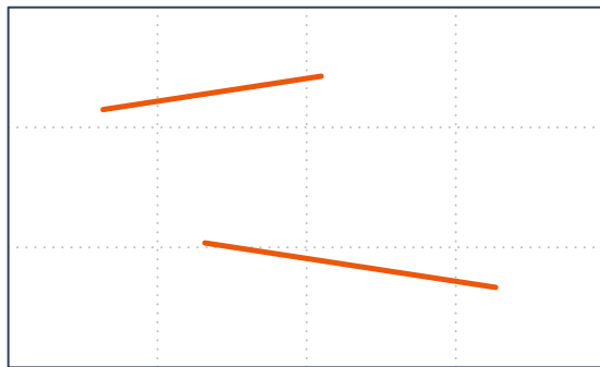
MultiLineString (Dim 1)
