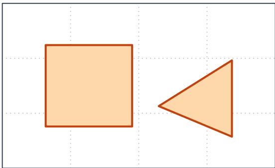
MultiPolygon (Dim 2)
