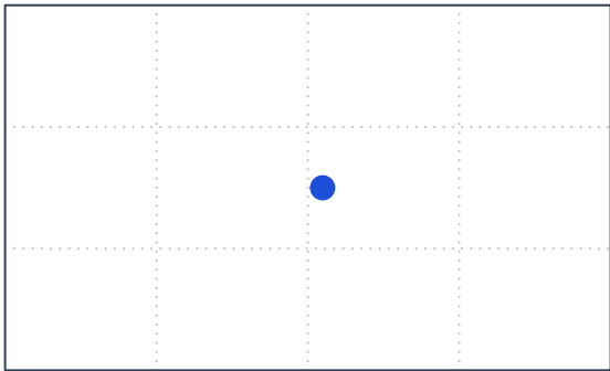
Point (Dim 0)
