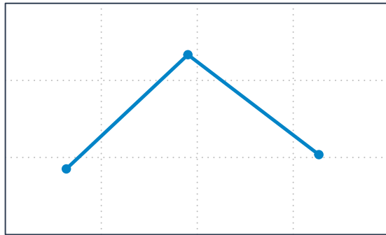
LineString (Dim 1)
