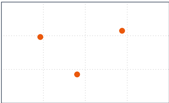
MultiPoint (Dim 0)
