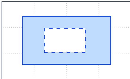
Polygon (Dim 2)
