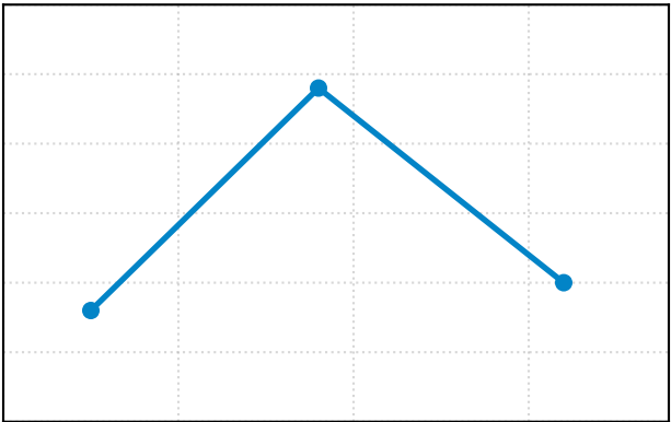
Polygon (Dim 2)
