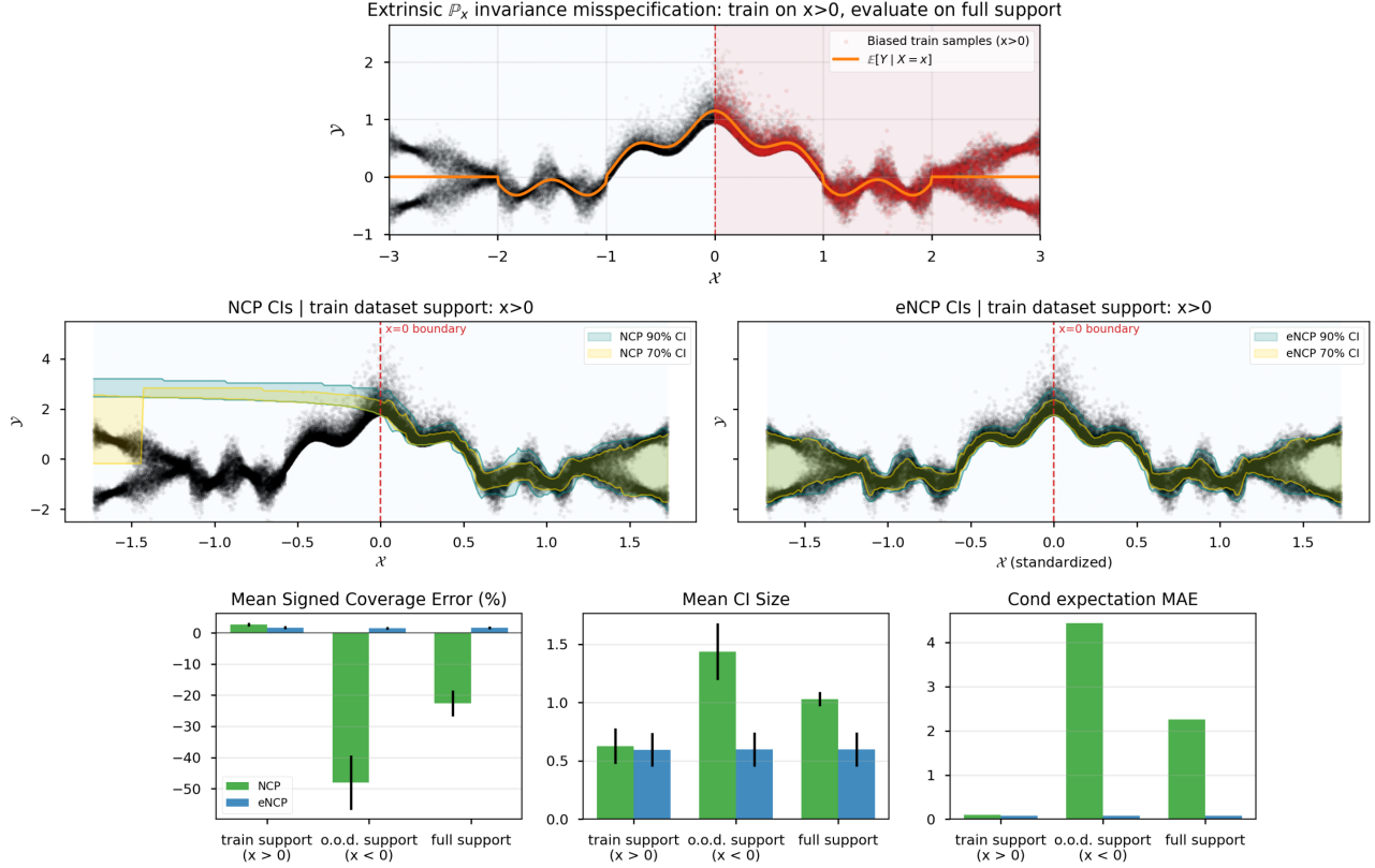
Figure A2. Top: Illustration of extrinsic symmetry misspecification, where the train/validation/test support is biased toward the coset subspace x > 0 , violating the assumed \mathbb{C}_2 -invariance of P_X . Middle: Predicted confidence intervals at 90% and 70% coverage for NCP and eNCP under extrinsic symmetry misspecification. Bottom: Mean coverage error, confidence-interval volume, and conditional-expectation Maximum Absolute Error (MAE) for NCP and eNCP, evaluated on the biased support x > 0 , the out-of-distribution (o.o.d.) support x < 0 , and the full support \mathcal{X} \equiv \mathbb{R} .
