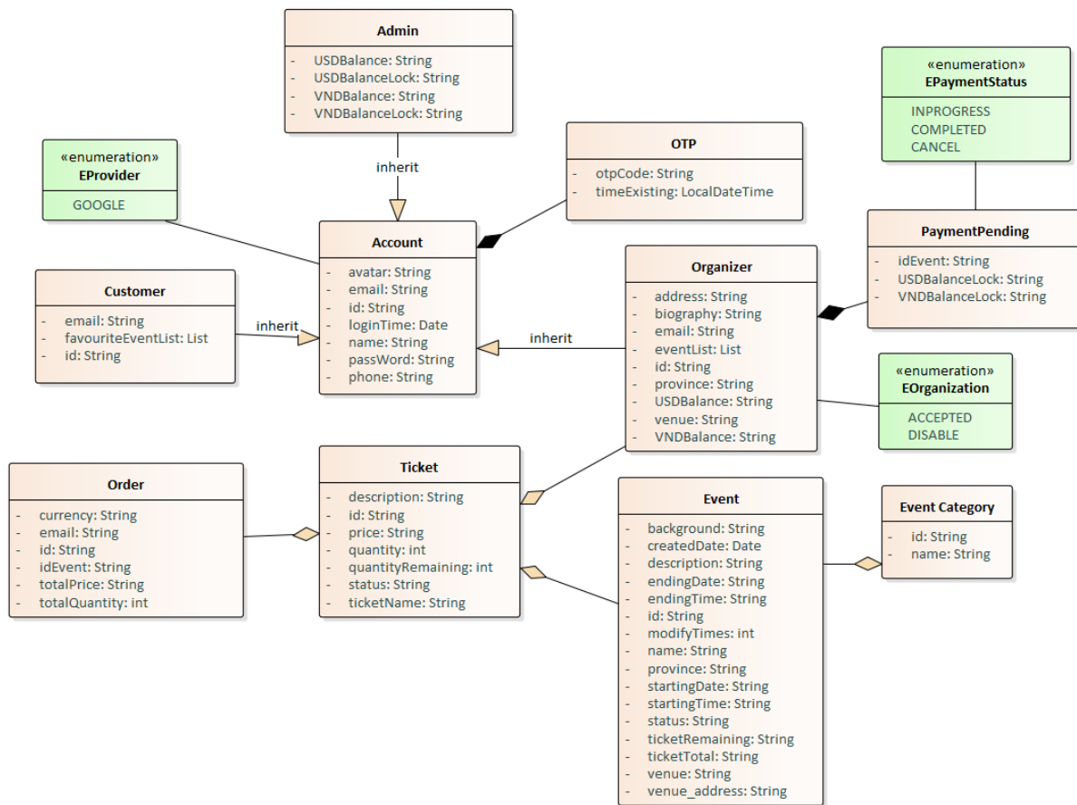
class Starter Class Diagram
