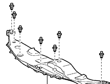
COOL AIR IN TAKE DUCT SEAL
