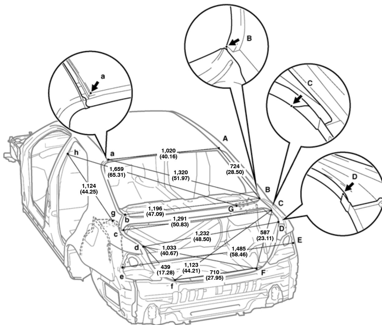
Vehicle Dimensions
