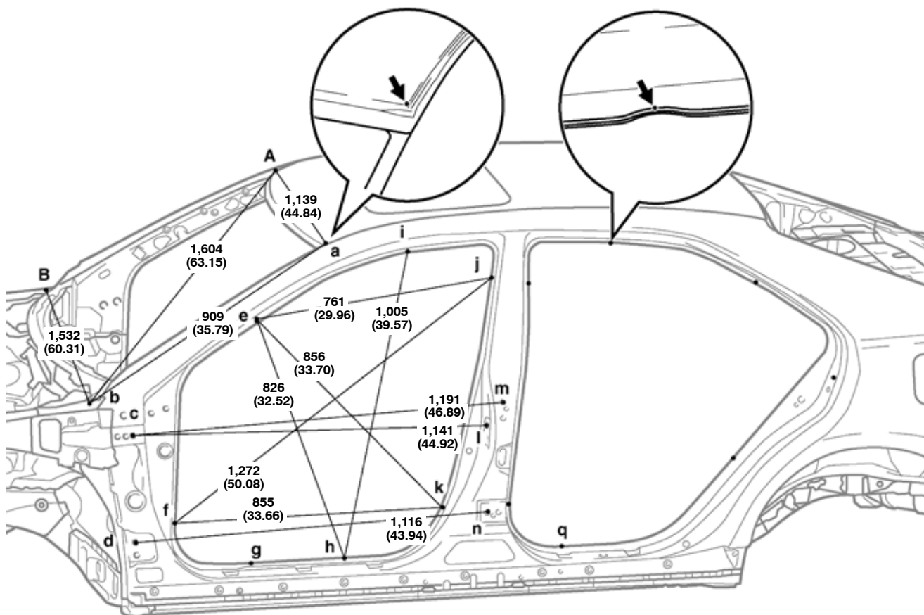
Vehicle Dimensions
