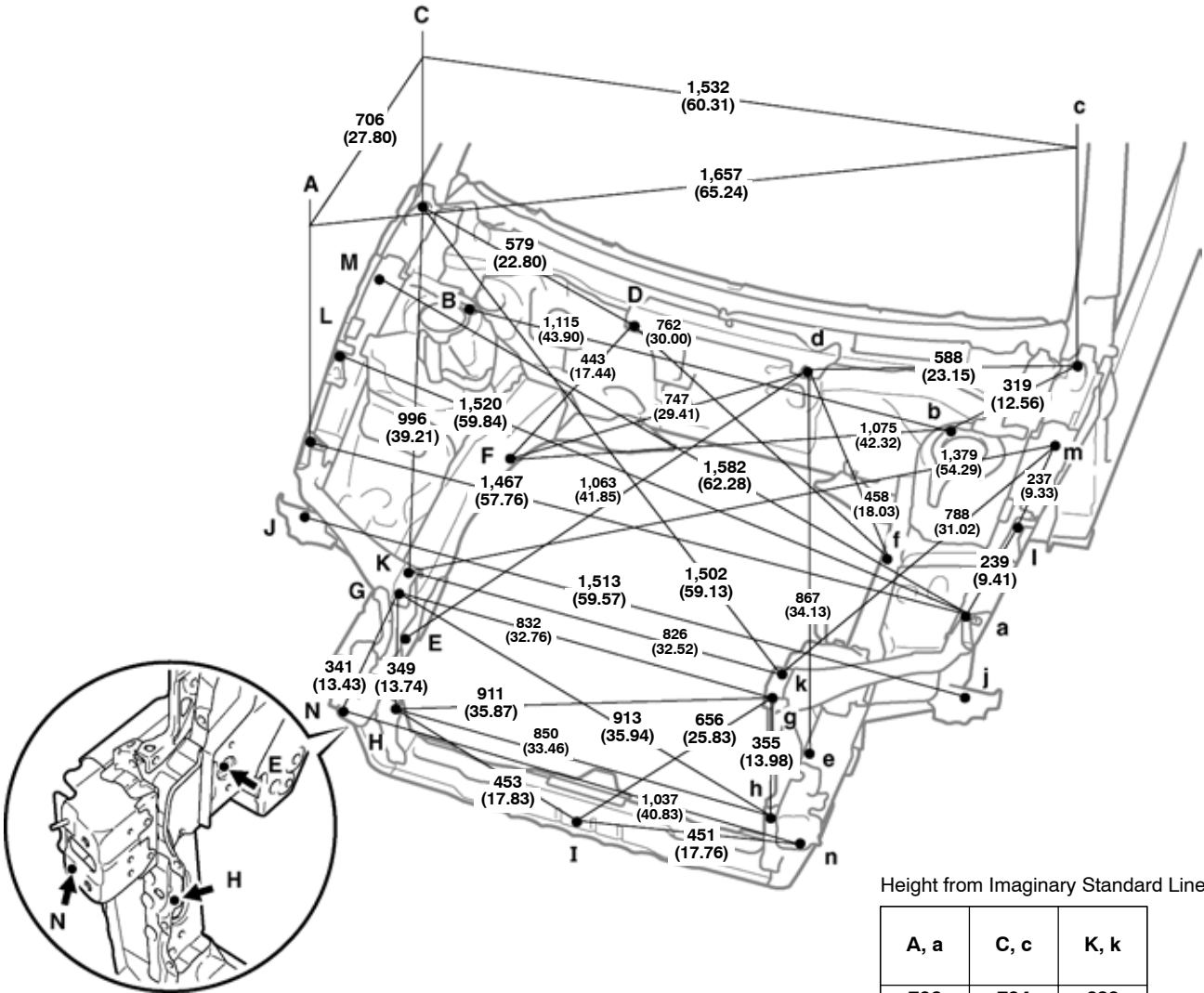
Vehicle Dimensions
