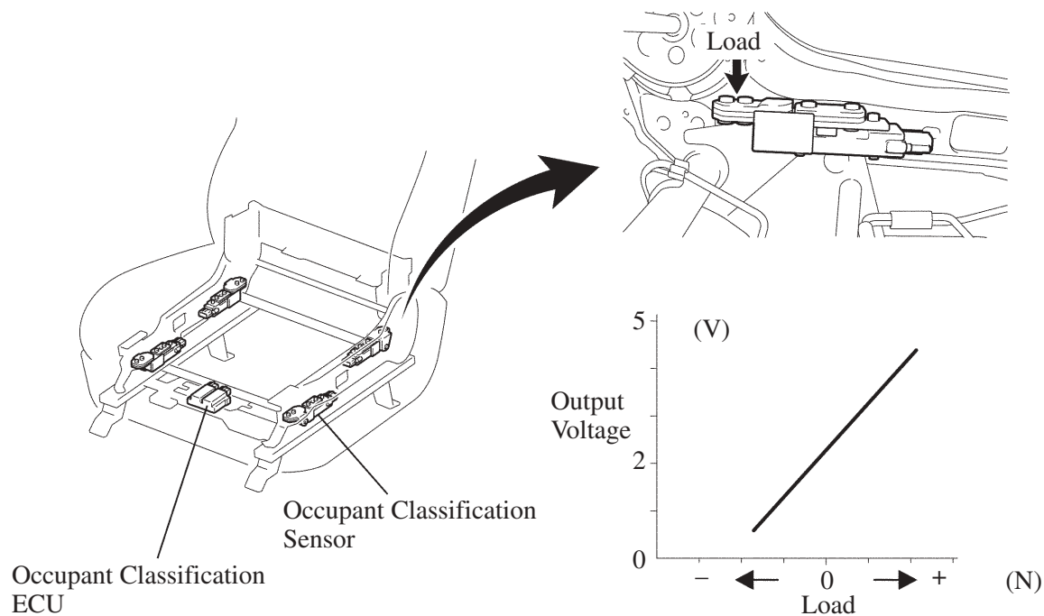
Relation between Output Voltage and Load
