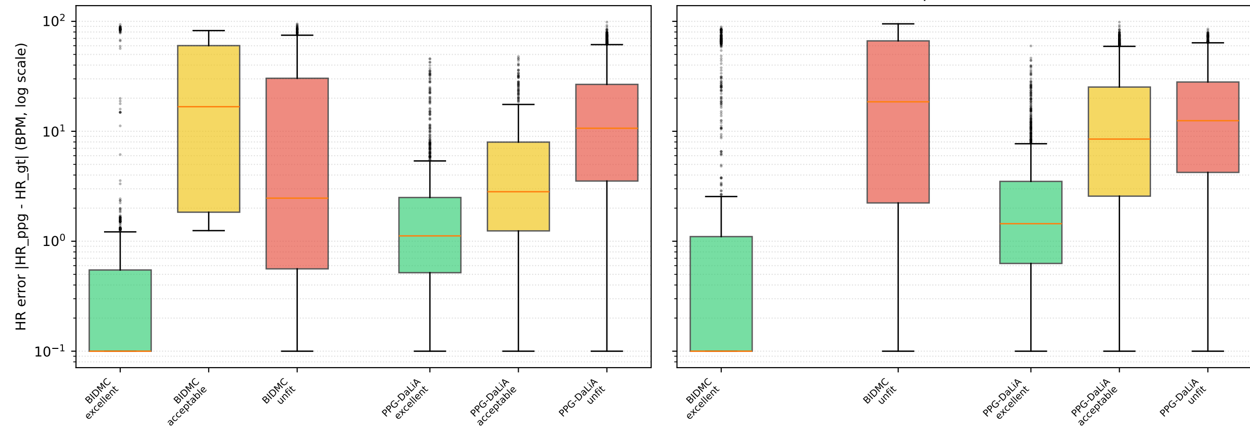
Pseudo-label tier
