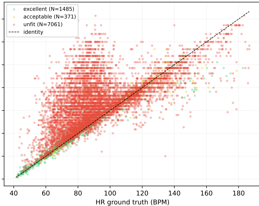
PPG-DaLiA
