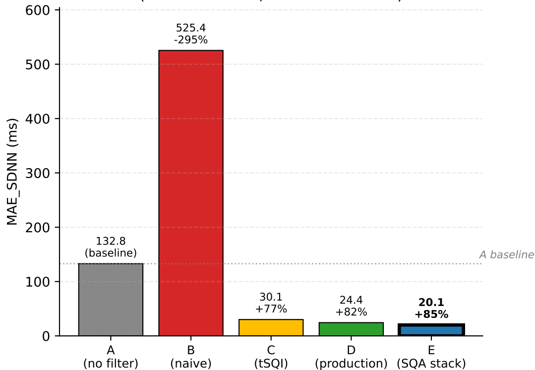
HRV SDNN MAE - 5-Method Comparison (PPG-DaLiA unfit, matched N=1871)
