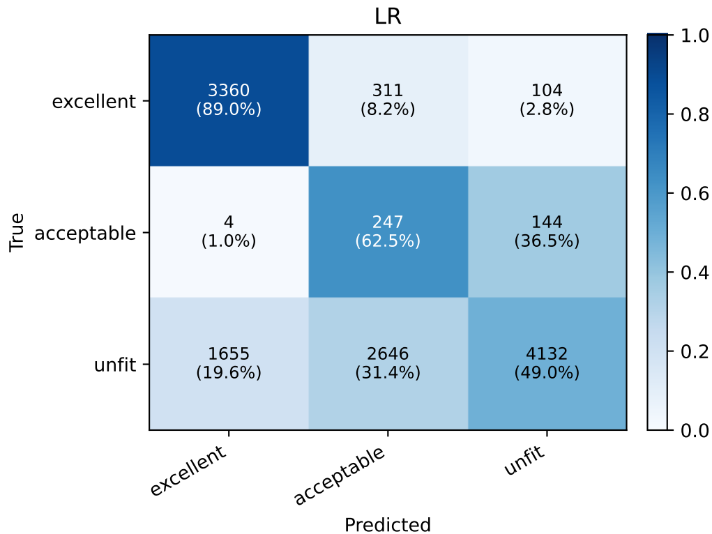
Confusion matrix (row-normalized): LR vs 3-criterion heuristic
