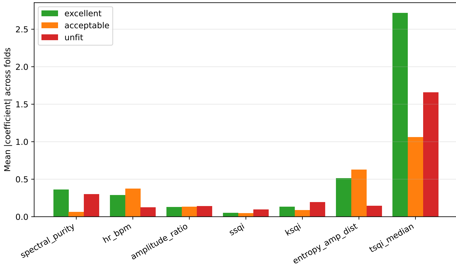
LR feature importance per class (StandardScaled inputs)
