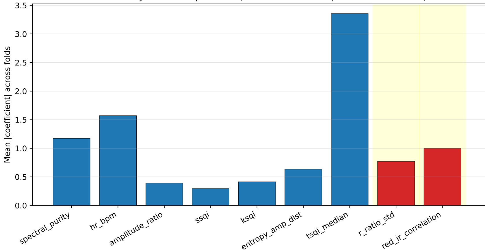
LR-9 binary feature importance (red bars = 2 new SpO2-aware features)
