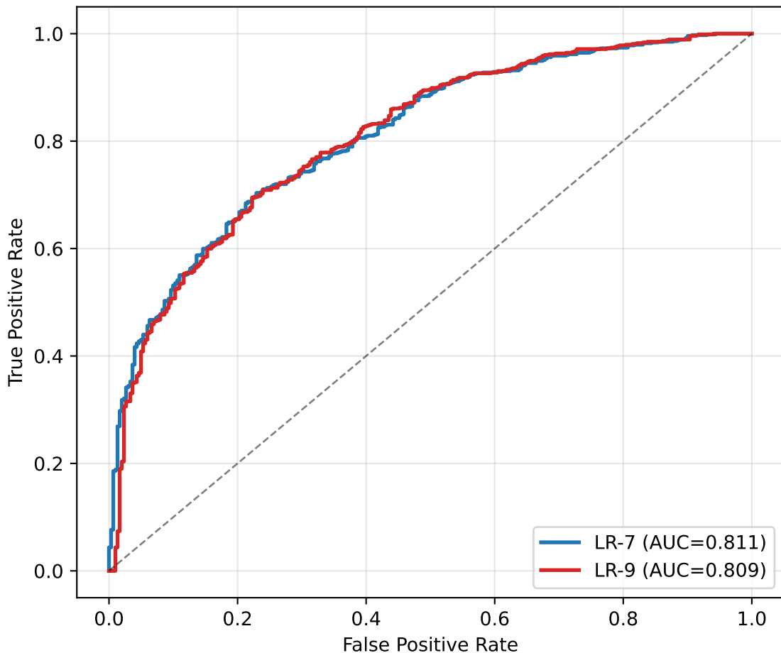
LR-7 vs LR-9 ROC (binary, BP+Quoc 1033 windows, GroupKFold) LR-7 AUC=0.811 LR-9 AUC=0.809
