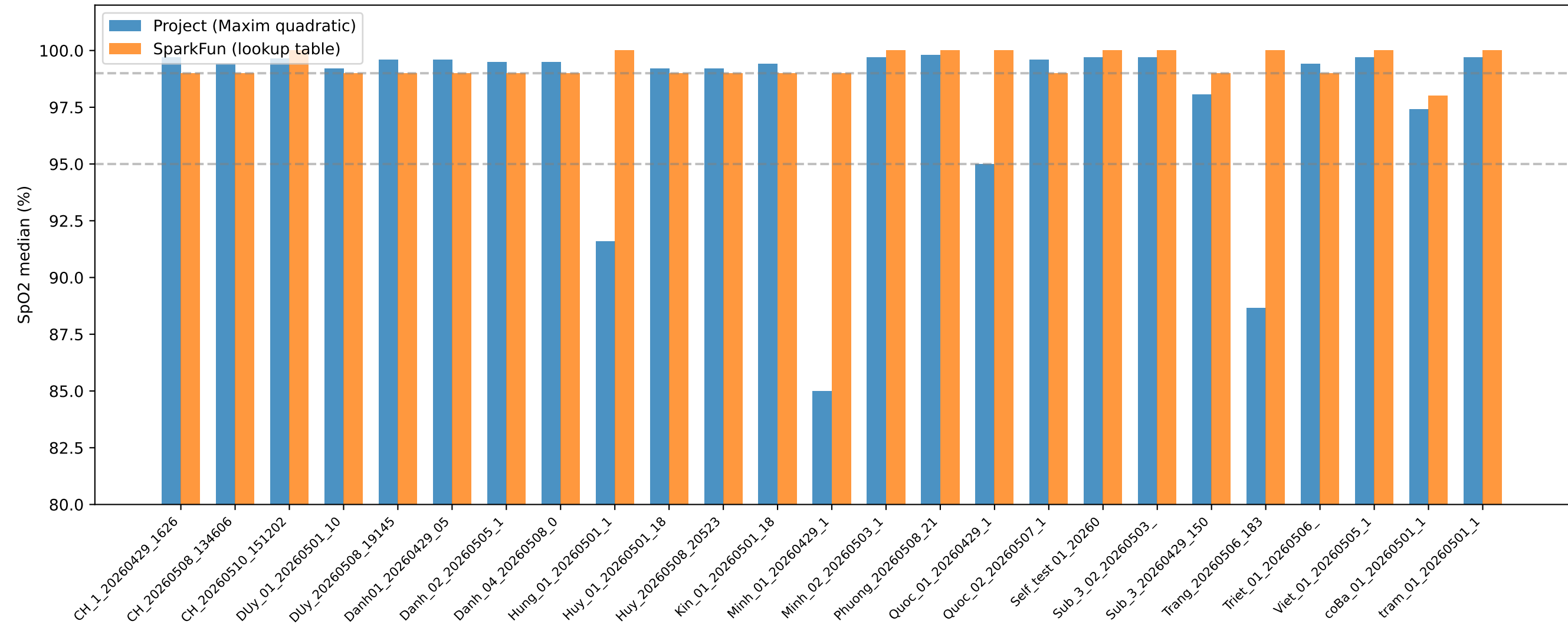
SpO2 per-subject: Project vs SparkFun chain on same samples
