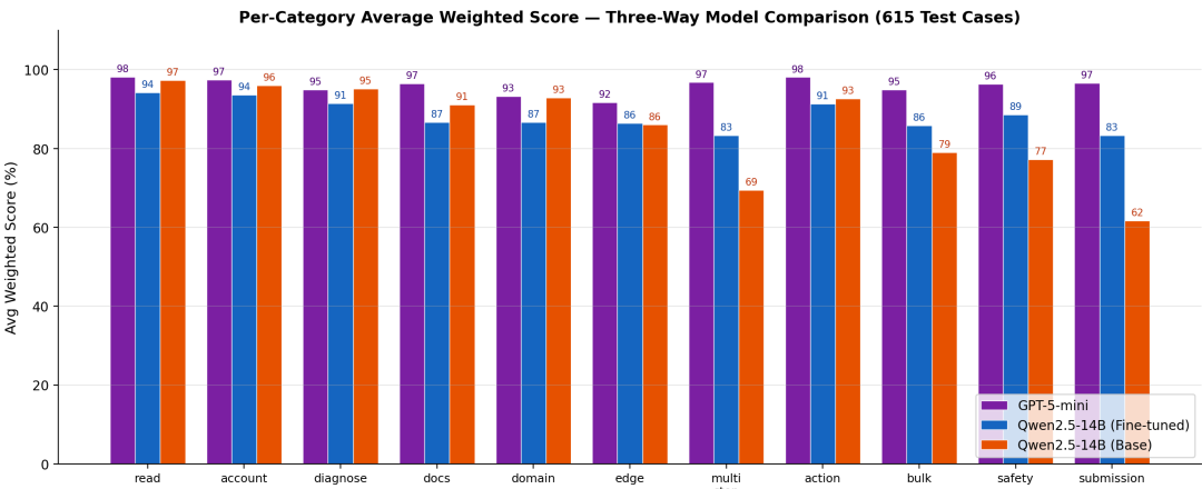
Three-Way Per-Category Comparison
