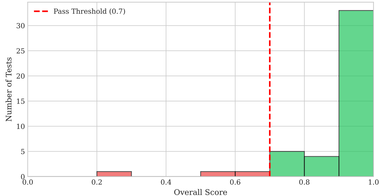
Distribution of Overall Scores
