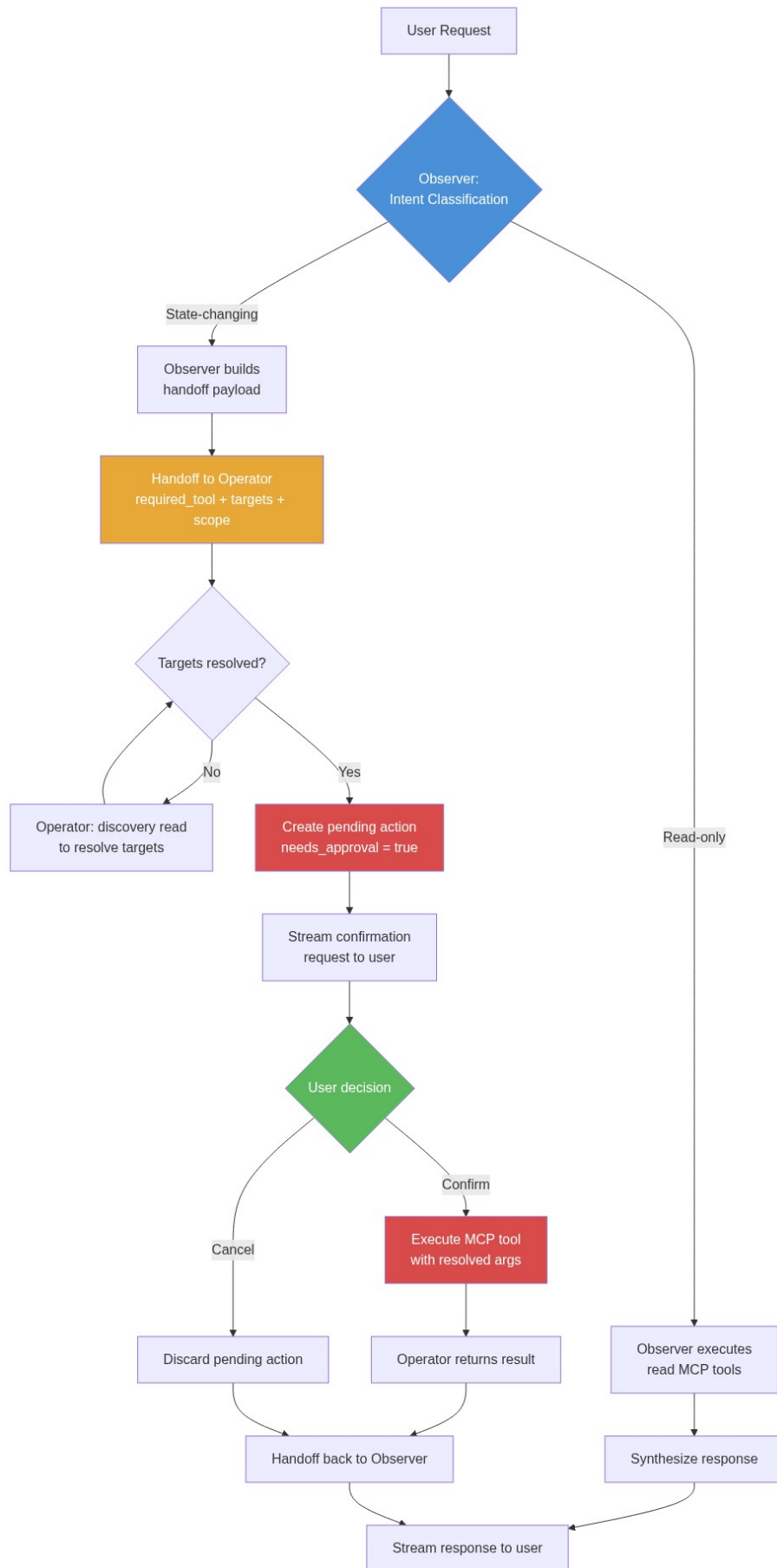
Figure 4.2: Observer/Operator Routing and Confirmation Flow
