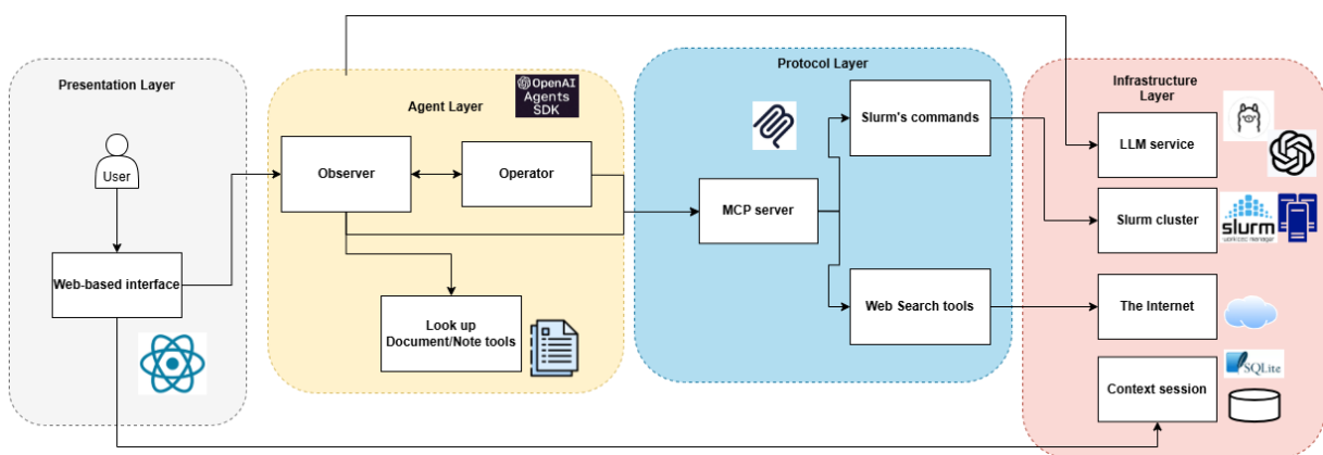
Figure 4.1: Slurm Agent System Architecture
