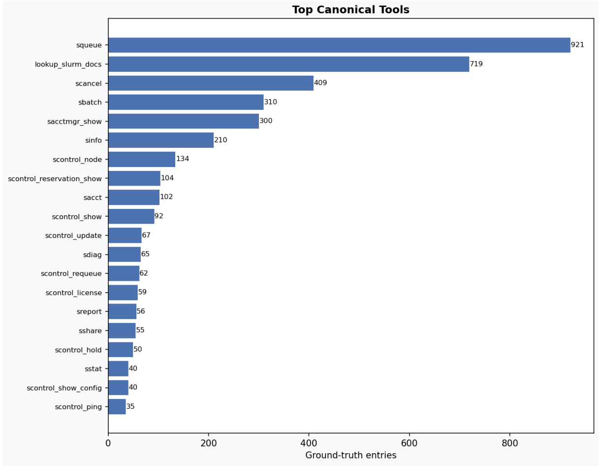
Figure 6.4: Tool Distribution After Normalization
