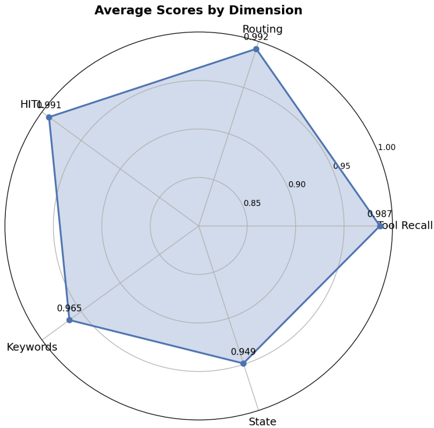
Figure 6.5: Aggregate Scoring Dimensions (Radar Chart)
