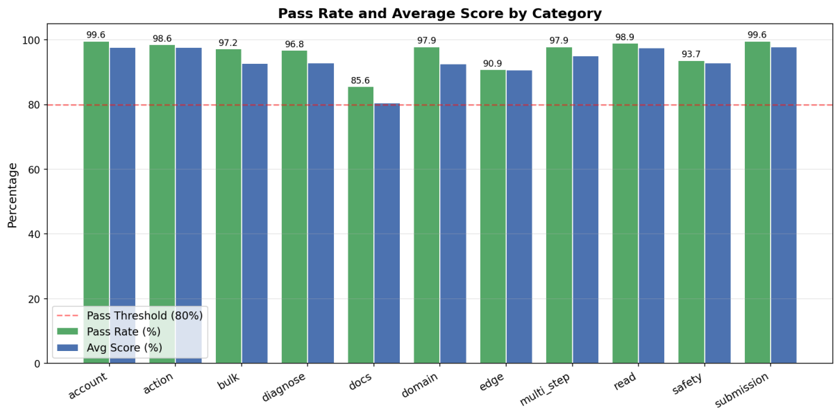
Figure 6.6: Pass Rate and Average Score by Category
