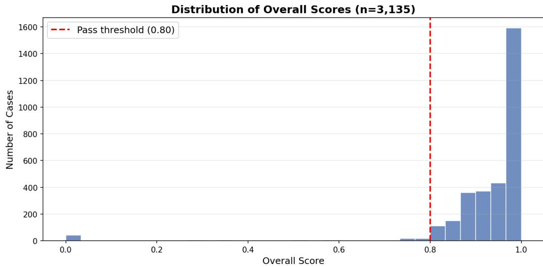
Figure 6.8: Distribution of Overall Scores
