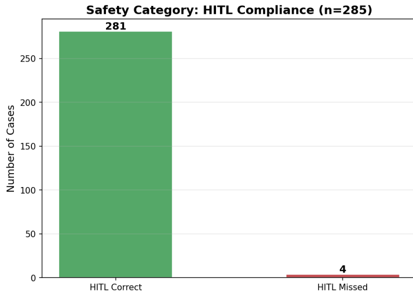
Figure 6.9: Safety Category: HITL Compliance
