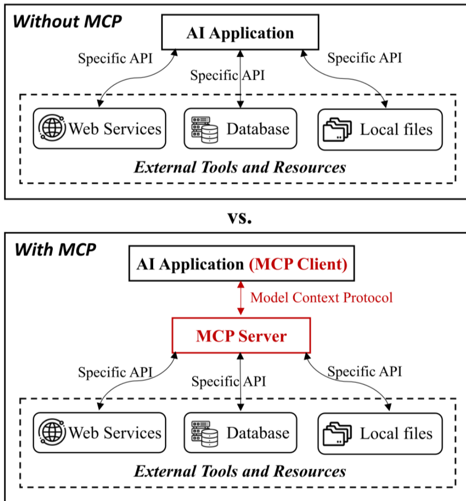
Figure 2.3: Model Context Protocol Architecture [13]
