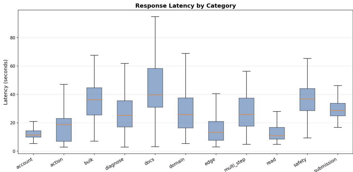
Figure 6.10: Response Latency by Category
