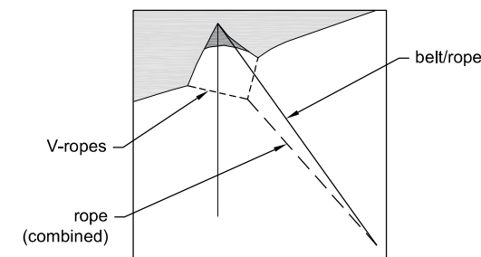
GUYING DIAGRAM [1:100]
