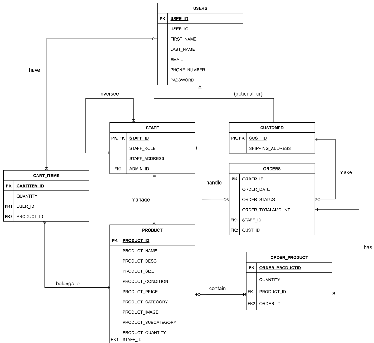
Figure 2.0: Entity Relationship Diagram (ERD) of ReWear Fashion System
