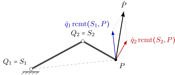
Figure 7: The Jacobian of a planar two-link arm acting on its tip P . In 2D the column of a revolute joint is its pivot point, S_j = Q_j ; each column contributes the velocity \dot{q}_j \text{rcmt}(S_j, P) , perpendicular to the lever from Q_j to P (dashed), and the tip velocity is their sum, eqn. (312).
