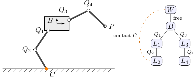
Figure 6: A robot model and its frame tree. A floating base B on a free joint carries two limbs of two links each, jointed at Q_1, \dots, Q_4 ; the lower limb touches the ground at C , the upper one carries a tool point P . The tree (right) reaches every frame from the world W on a unique path; the contact is a constraint between the last link and the world (dashed), which closes a loop while it is active.
