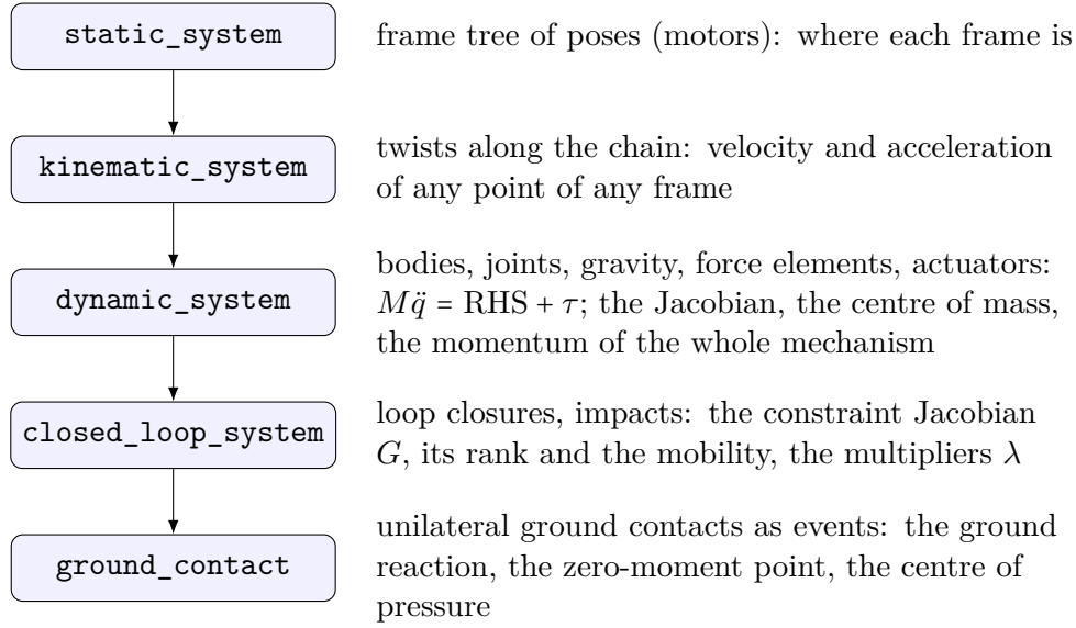
Figure 5: The mechanics layer as a stack. Each class builds on the one above it and adds one kind of state; the right column lists what a robotics application reads from each layer.
