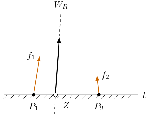
Figure 9: The zero-moment point in 2D . The contact forces f_1, f_2 at P_1, P_2 sum to the reaction wrench W_R , which is the line of action of their resultant (dashed, resultant force drawn bold); Z = W_R \vee L is where that line meets the ground.
