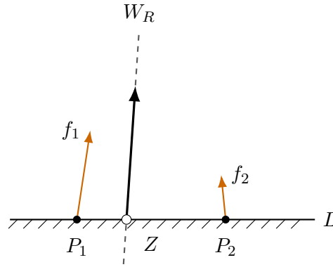
Figure 9: The zero-moment point in 2D . The contact forces f_1, f_2 at P_1, P_2 sum to the reaction wrench W_R , which is the line of action of their resultant (dashed, resultant force drawn bold); Z = W_R \vee L is where that line meets the ground.
