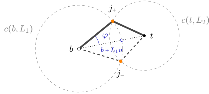
Figure 8: Two-link inverse kinematics by both routes. PGA : the point b + L_1 u on the line from b to t (dotted), turned about b by \pm\varphi (eqn. (318)). CGA : the joint lies on both circles, so the dipole c(b, L_1) \vee c(t, L_2) carries both configurations j_{\pm} (solid and dashed). A tip out of reach gives |\cos\varphi| > 1 in the one route and an imaginary radius of the dipole in the other.
