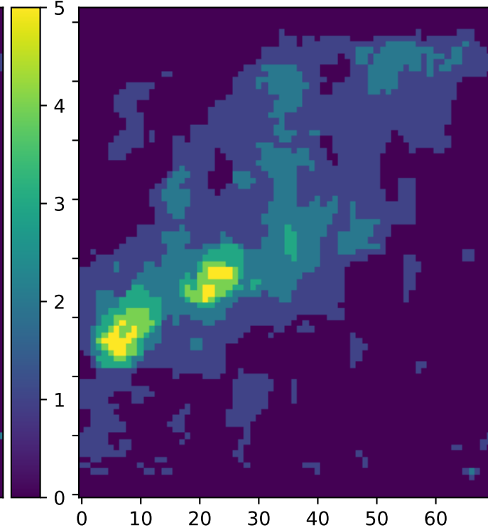
Gaussian Blur
