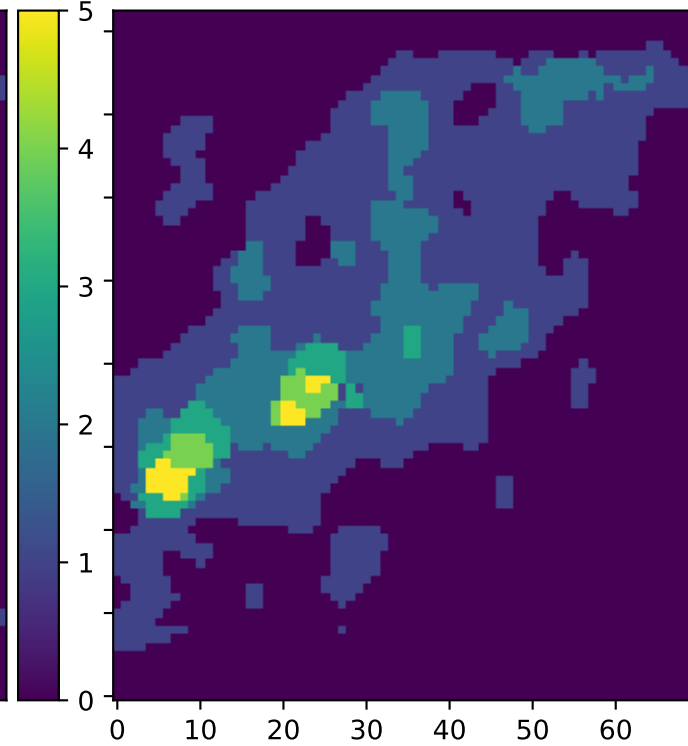
Mode Filter
