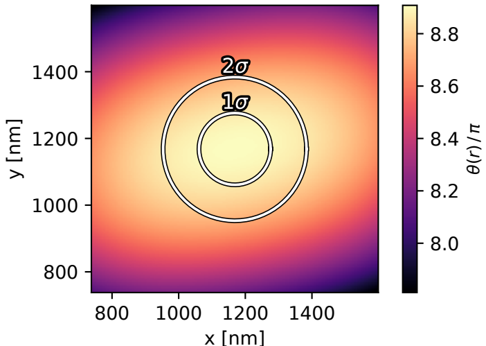
Pulse area point by point - no averaging anywhere white: 1 and 2 sigma of the atomic position distribution
