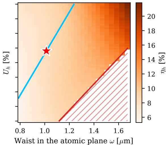
Crosstalk \eta_h (hard metric)
