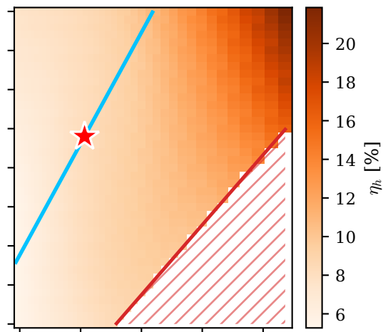
Amplitude ratio r_y
