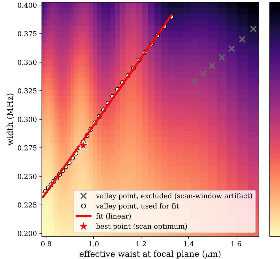
Crosstalk (fixed-amplitude scan)
