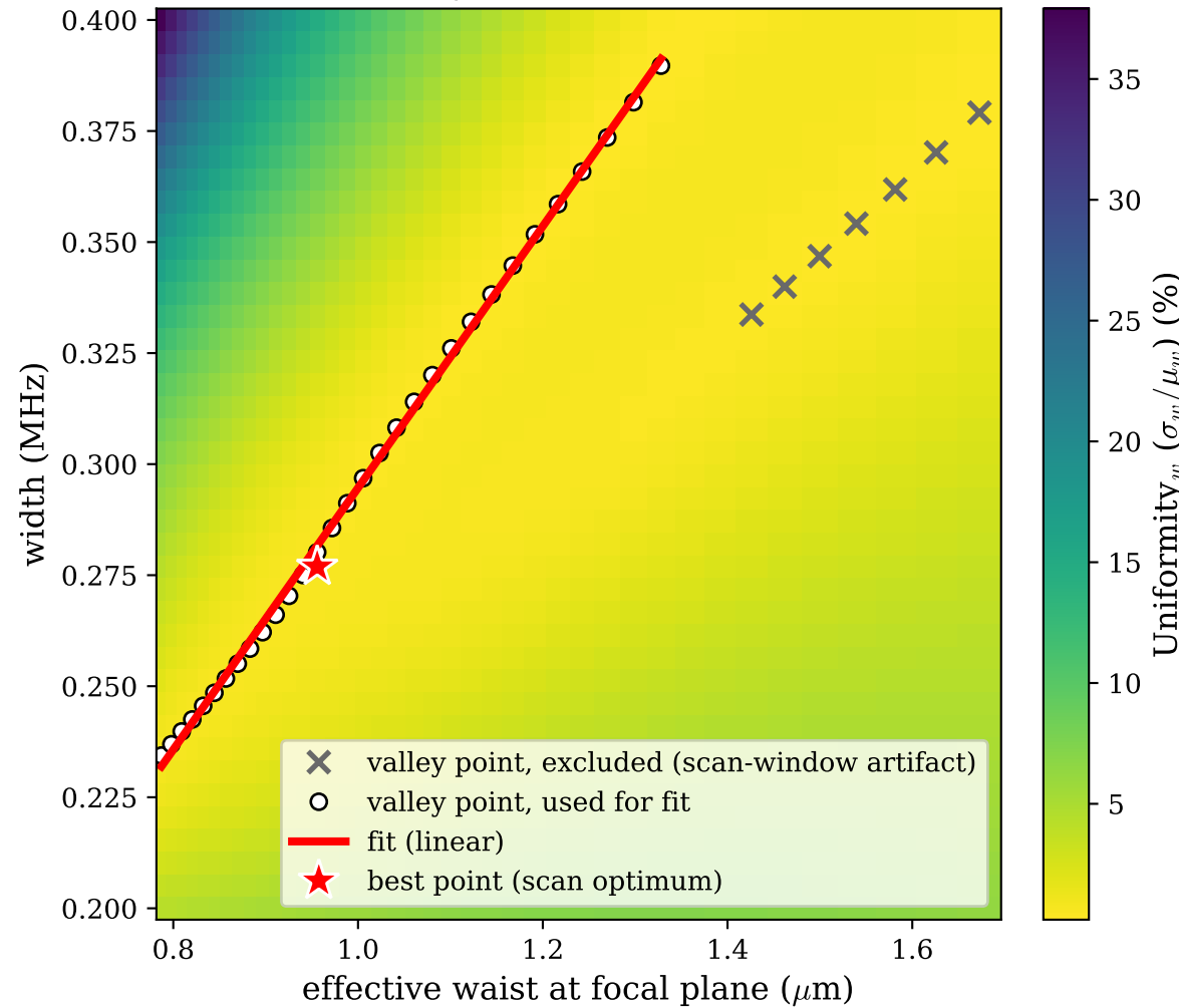
Uniformity (fixed-amplitude scan)
