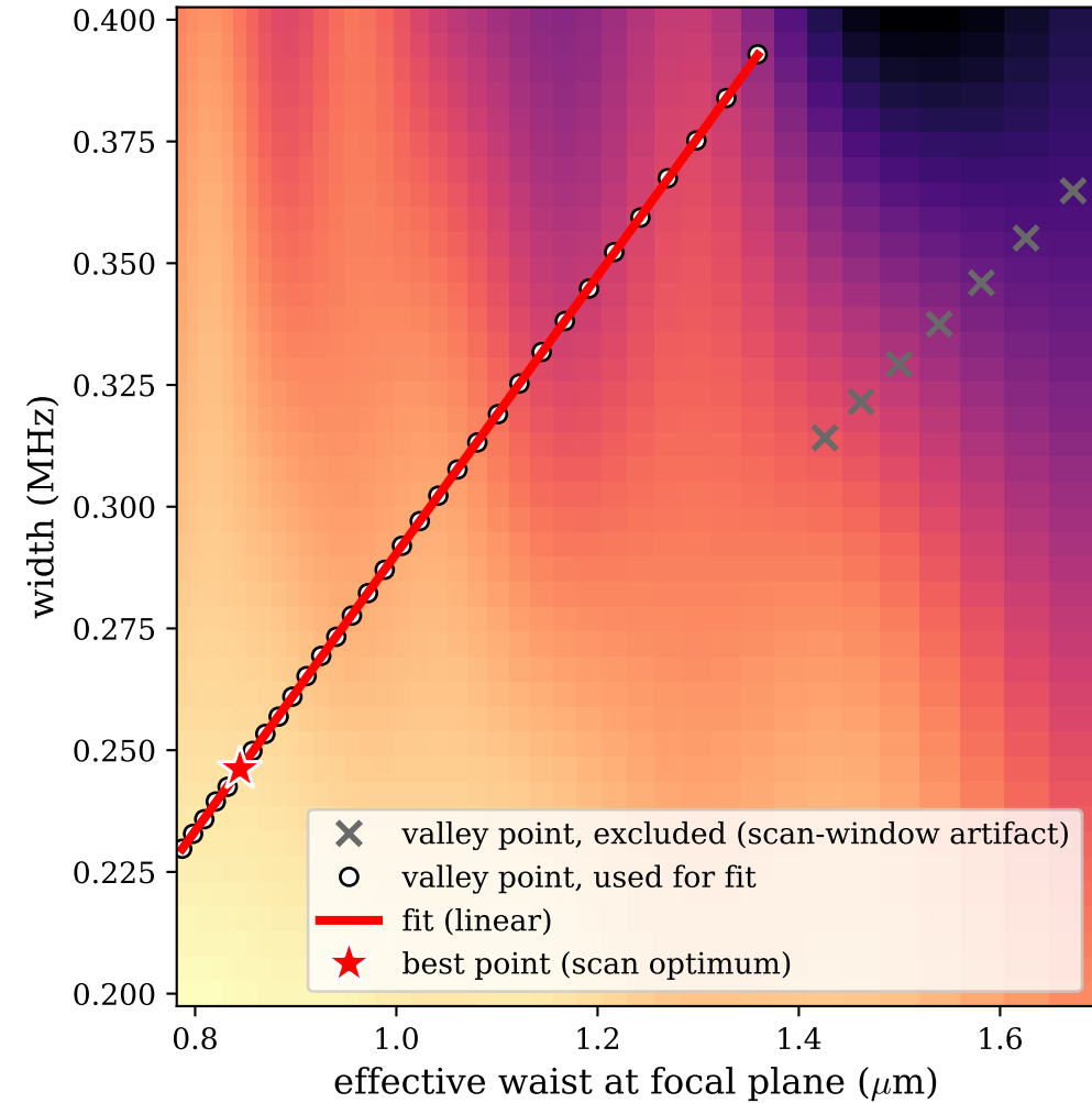
Crosstalk (fixed-amplitude scan)
