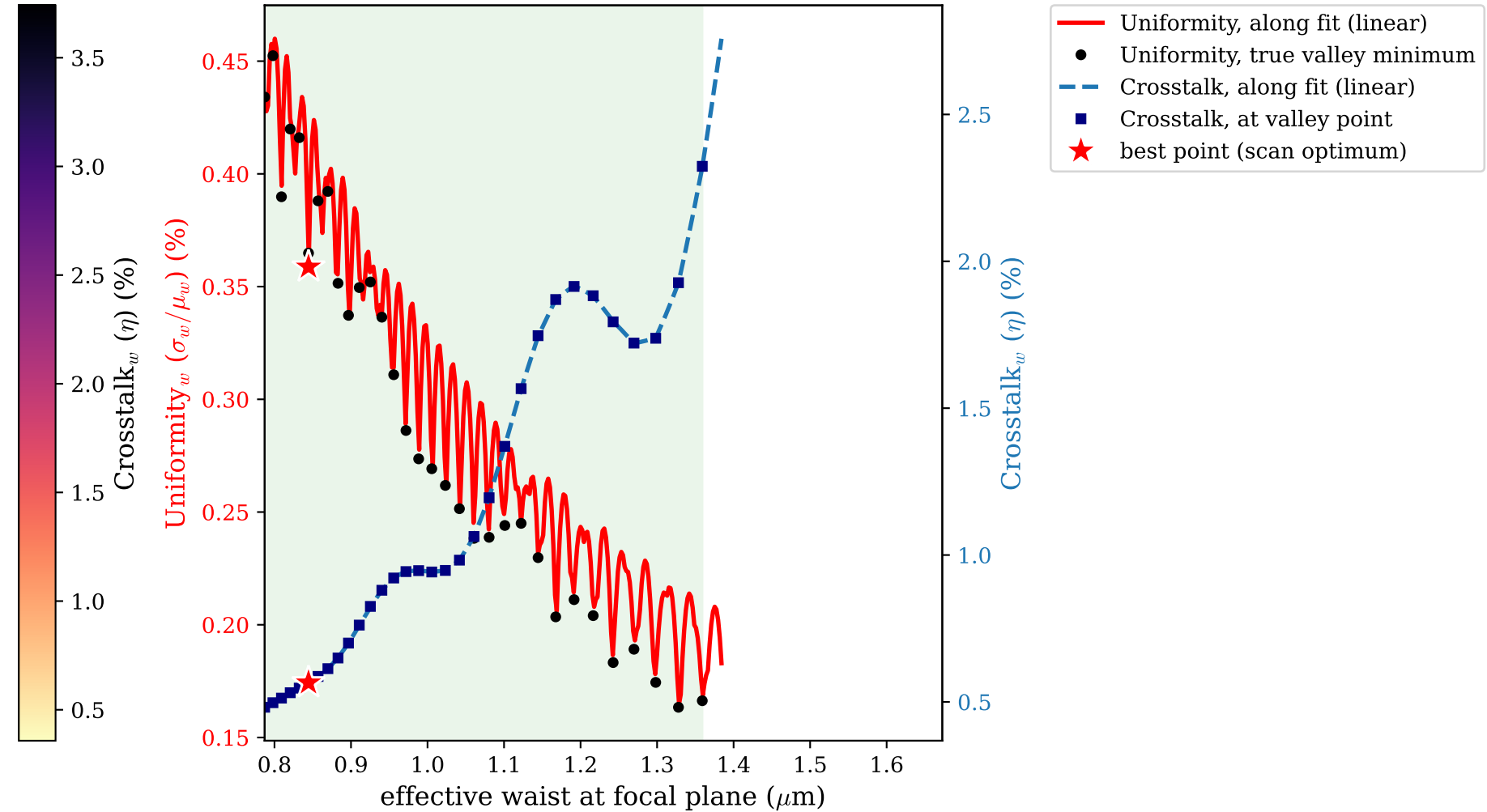
Uniformity / Crosstalk cut along the fitted line
