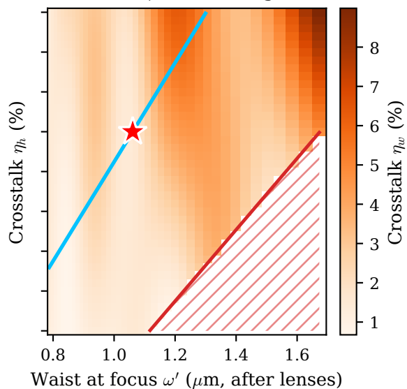
Crosstalk \eta_w (atom-weighted)
