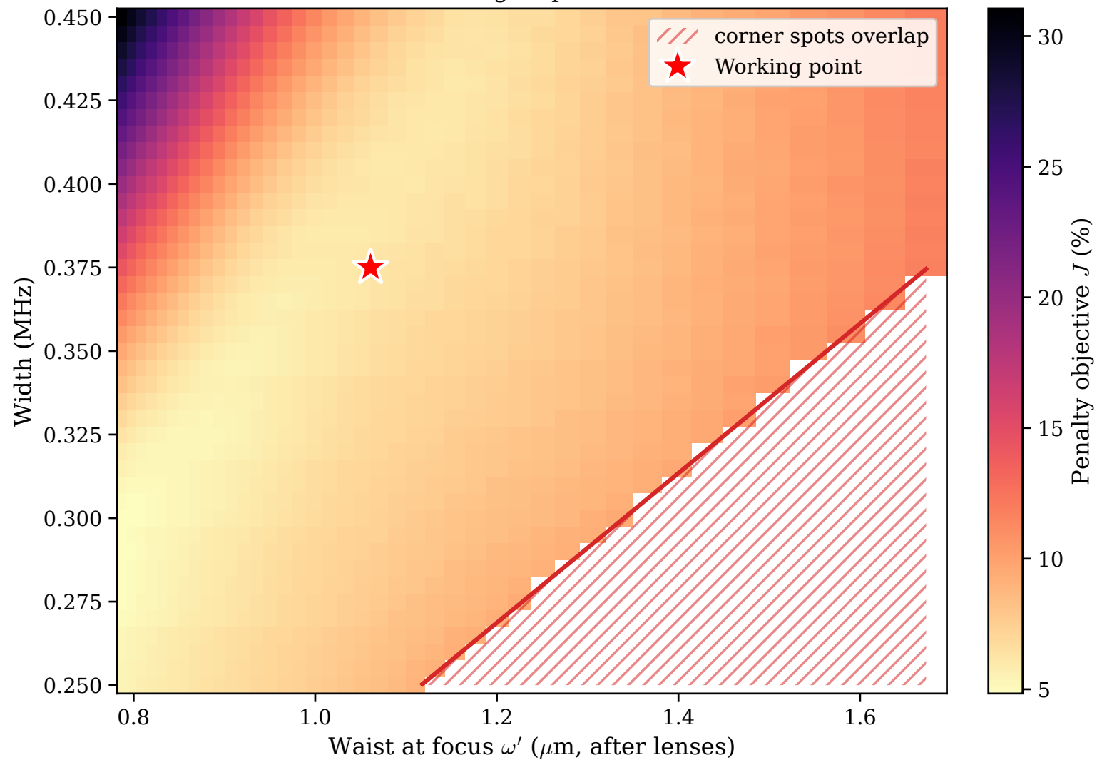
Penalty region best 25% of all grid points: 368/1681
