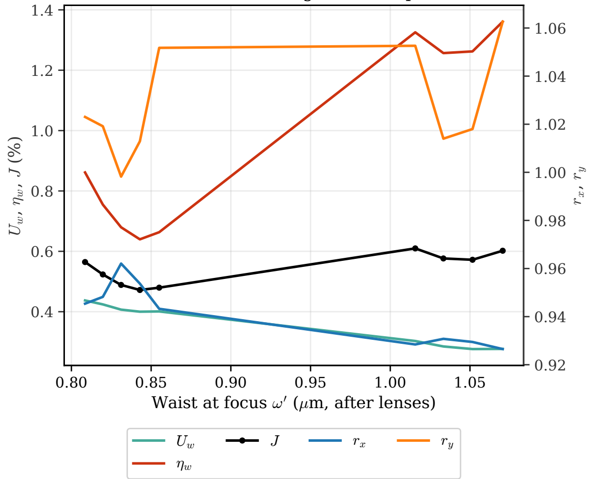
Cross-section along minimum path
