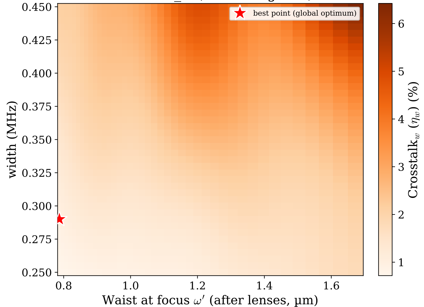
Crosstalk_w (atom-weighted)
