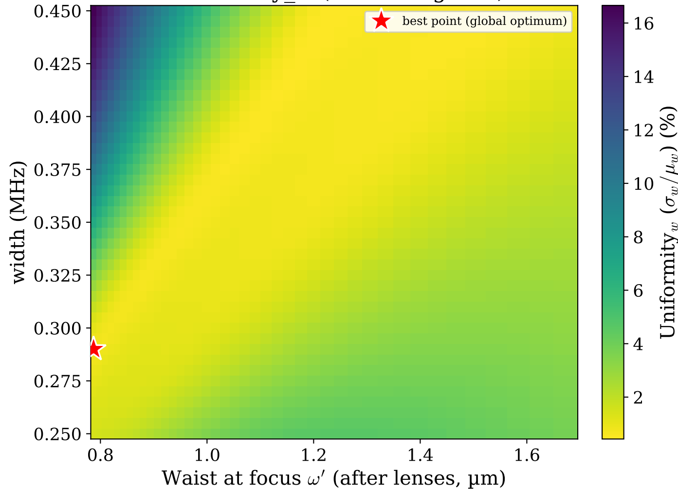
Uniformity_w (atom-weighted)
