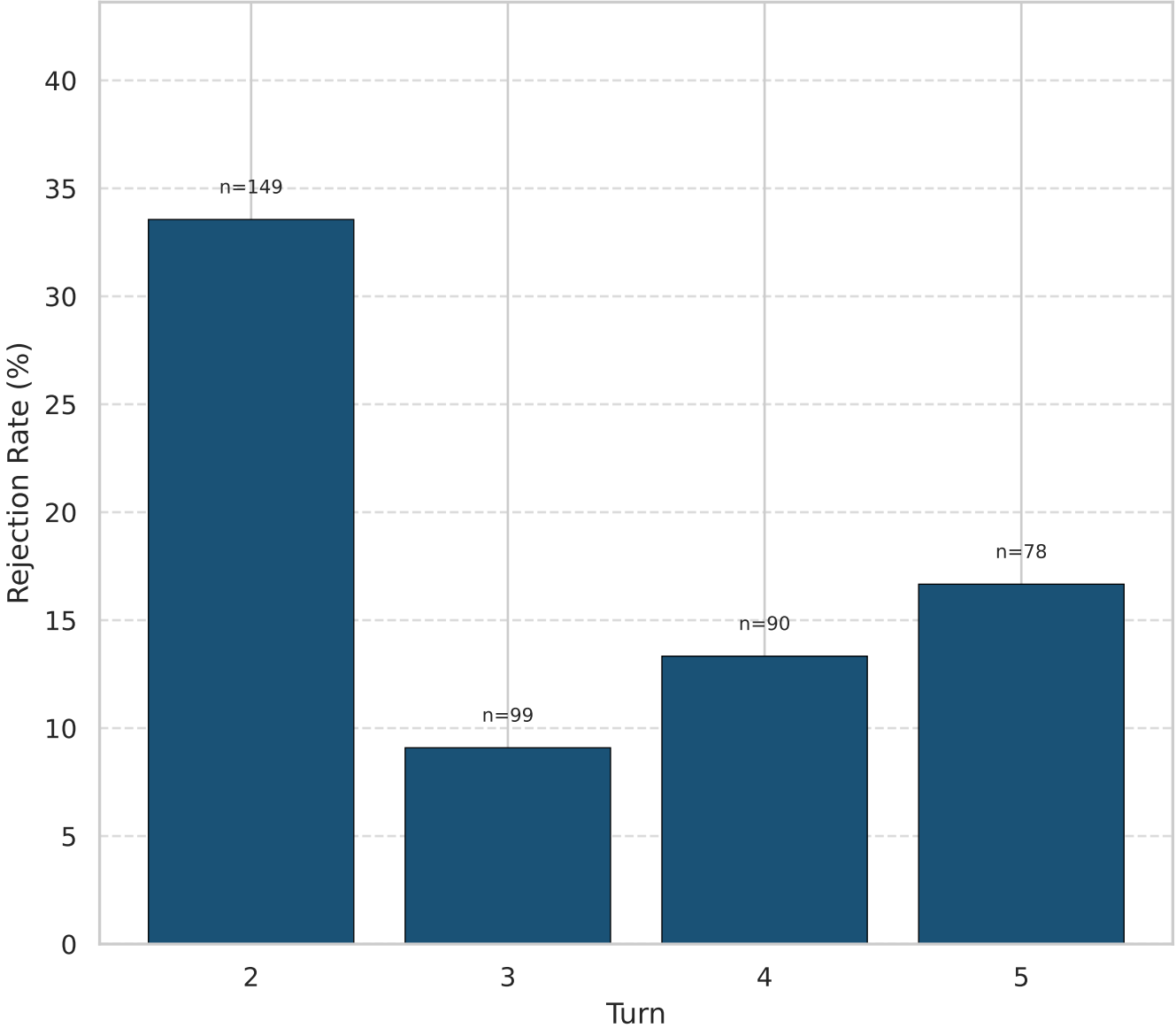
Cache Rejection Rate per Turn
