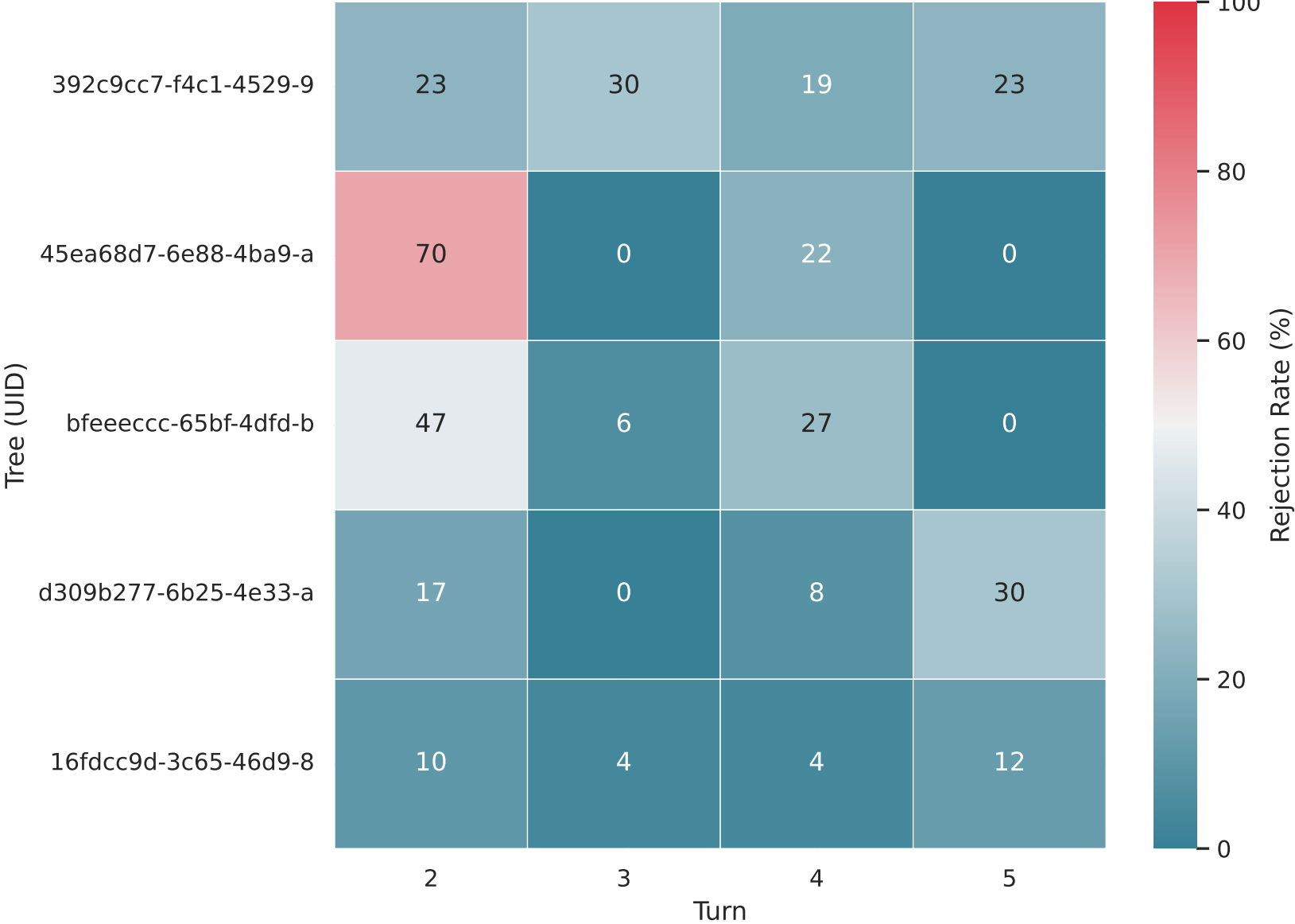
Cache Rejection Rate: Tree × Turn
