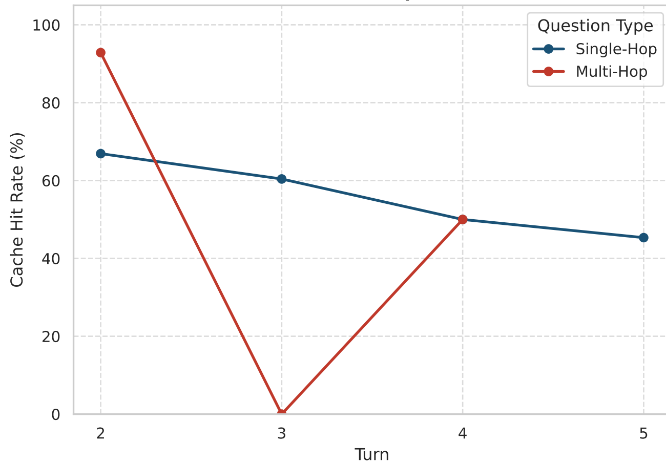
Cache Hit Rate per Turn
