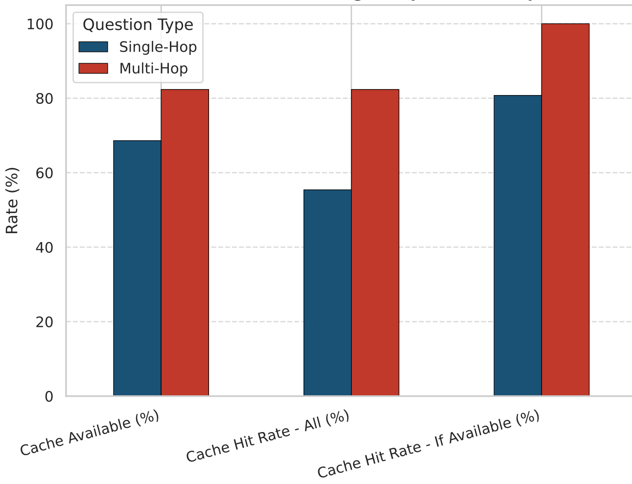
Cache Likelihood: Single-Hop vs Multi-Hop
