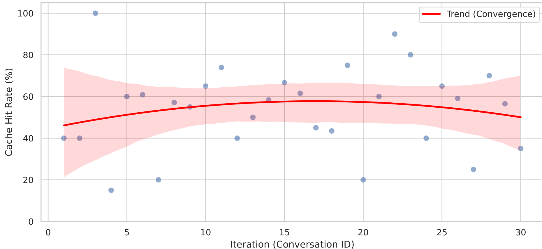
Cache Convergence in CI/CD Simulation (30 Iterations)
