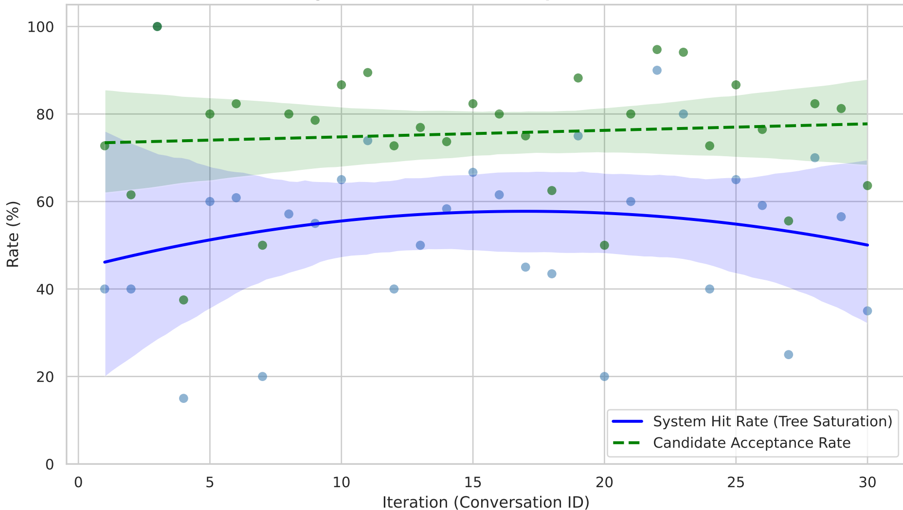
Cache Convergence and Candidate Acceptance in CI/CD Simulation
