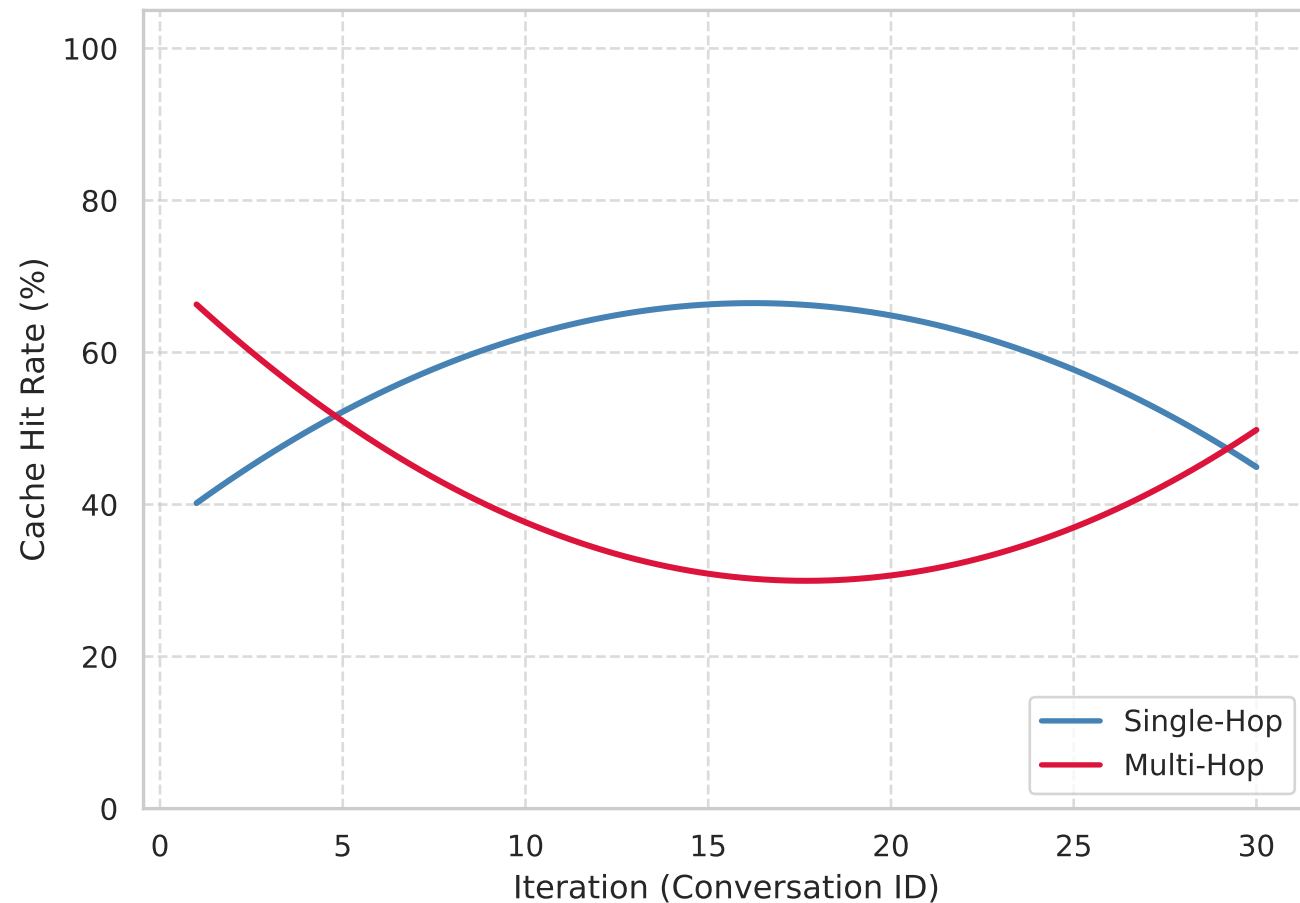
Cache Hit Trend over Iterations
