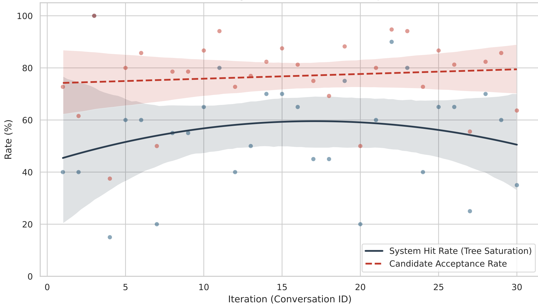
Cache Convergence and Candidate Acceptance
